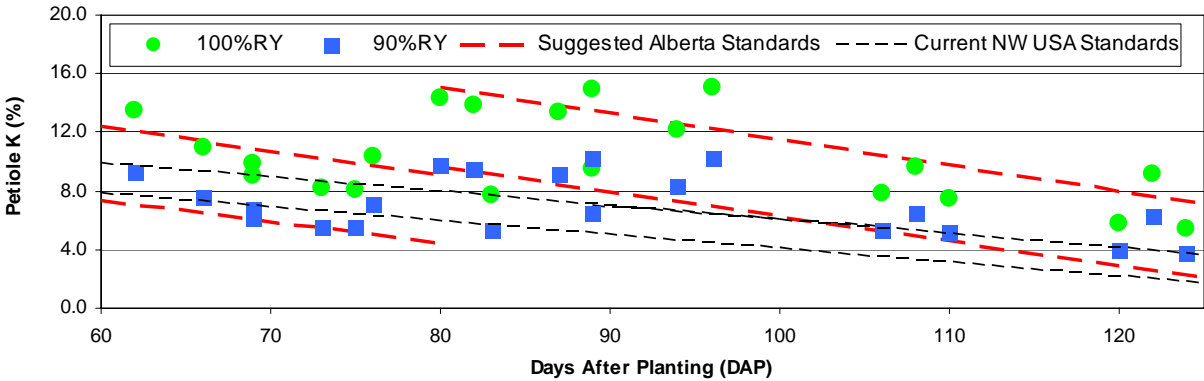
Figure 17. Suggested optimal petiole NO 3 -N, P, and K concentrations for southern Alberta compared to current northwest USA recommendations and to the 100%RY and 90%RY data collected in 2004, 2005, and 2007.
